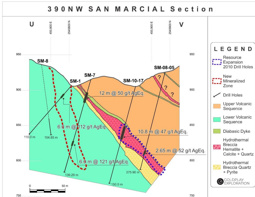
Figure 6: San Marcial Cross Section U-V
