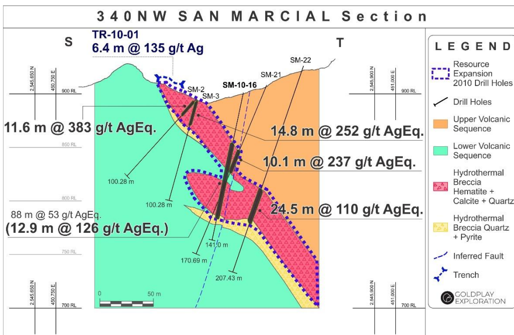
Figure 6: San Marcial Cross Section S-T
