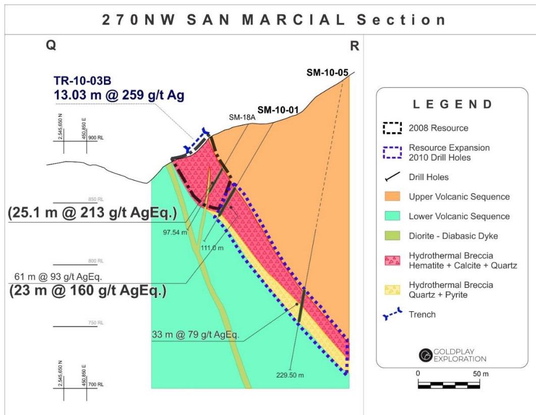
Figure 2: San Marcial Cross Section Q-R
