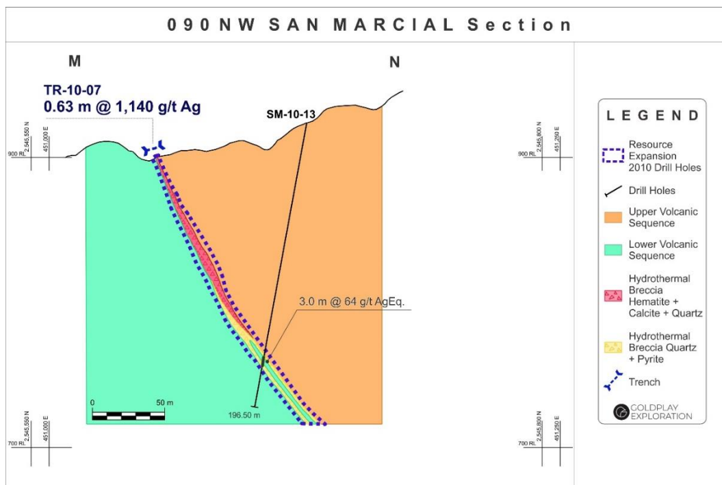
Figure 4: San Marcial Cross Section M-N
