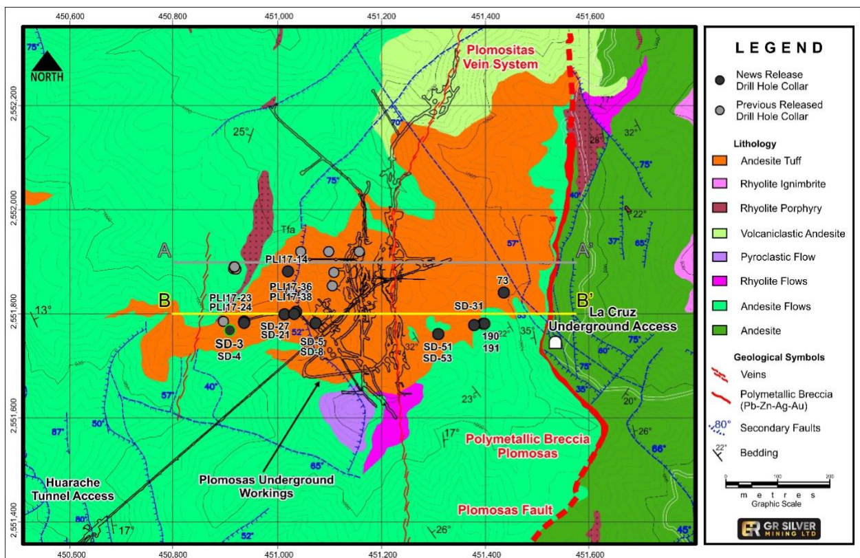
Figure 2: Drill Hole Collar Locations– Mineralized Structures (Plomosas Mine Area)
