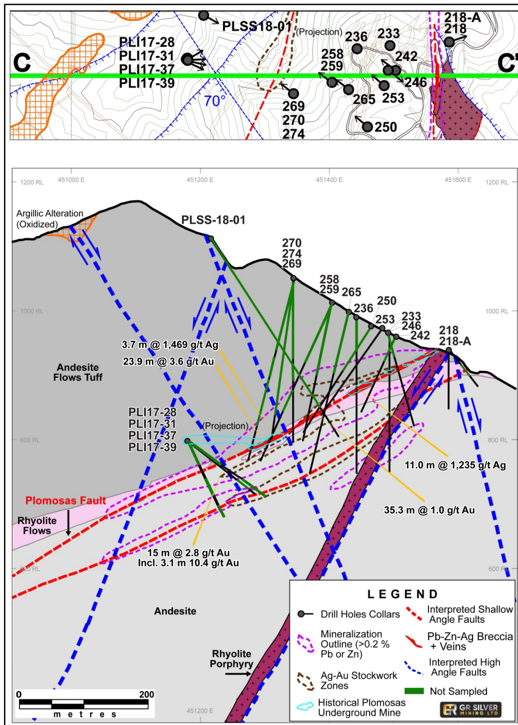
Figure 2: Cross Section - News Release 22/6/2020 - Drill Hole Collar Locations – Mineralized Structures (Plomosas Mine Area)
