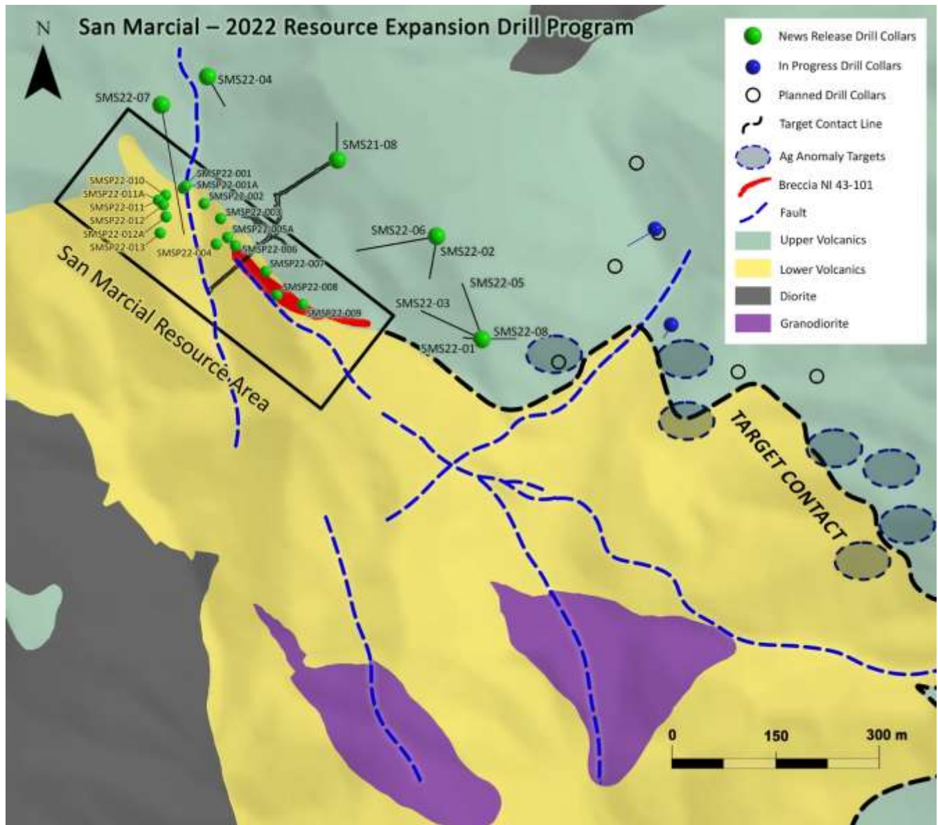
Figure 2: Location of 2022 Drill Holes and SE Extension Target Contact Zone
