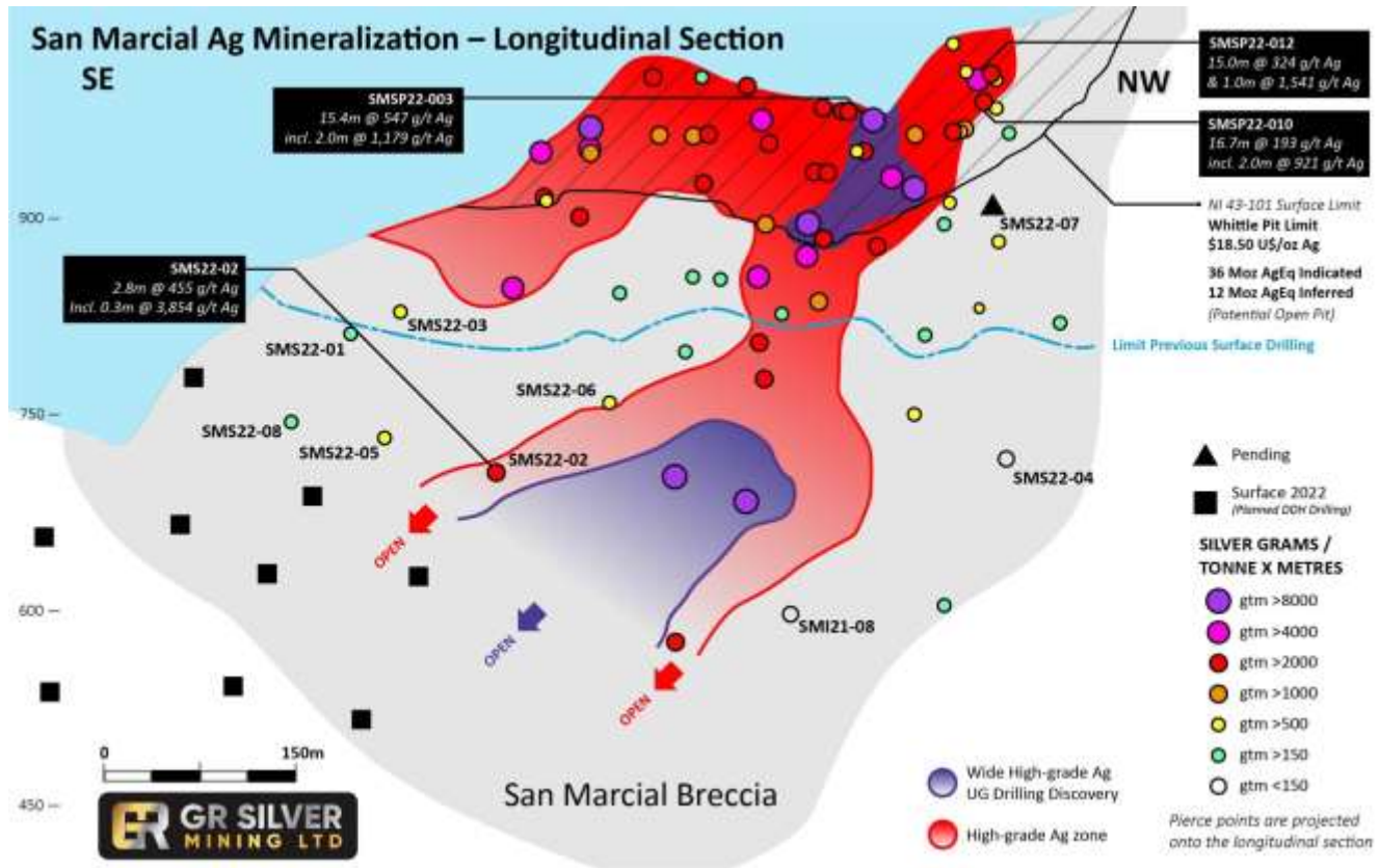
Figure 1: San Marcial Longitudinal Section – Drilled Pierce Points with Grade x Thickness
